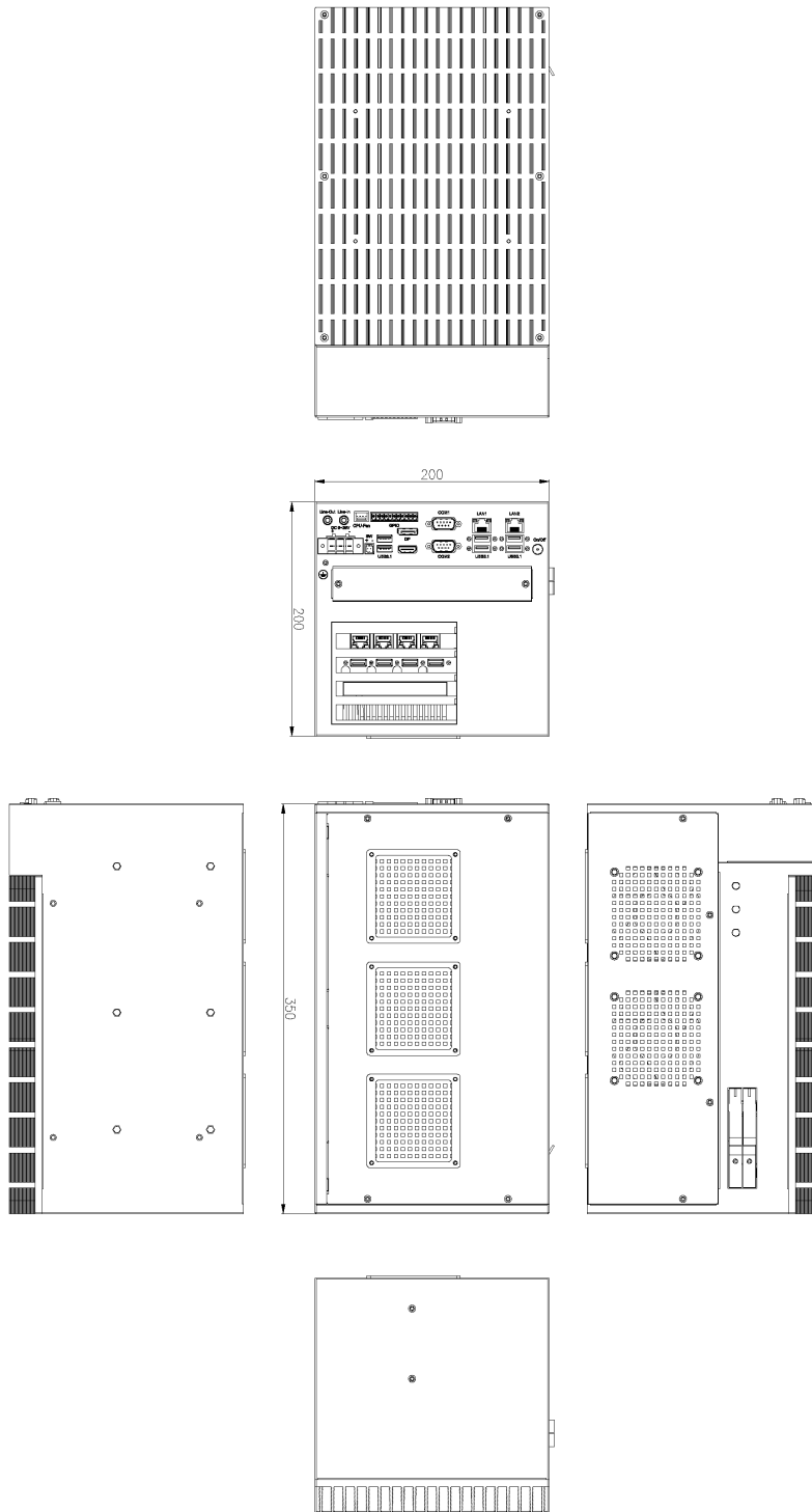
Figure 1.1: Dimension of TB-5745
