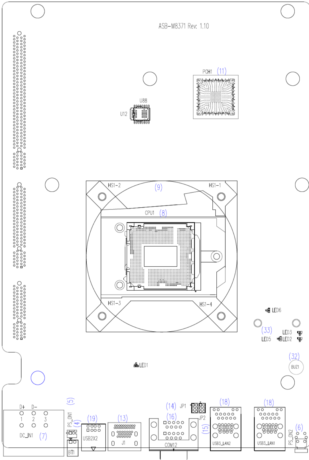
Figure 2.2: Jumpers and Connectors Location- Board Top
