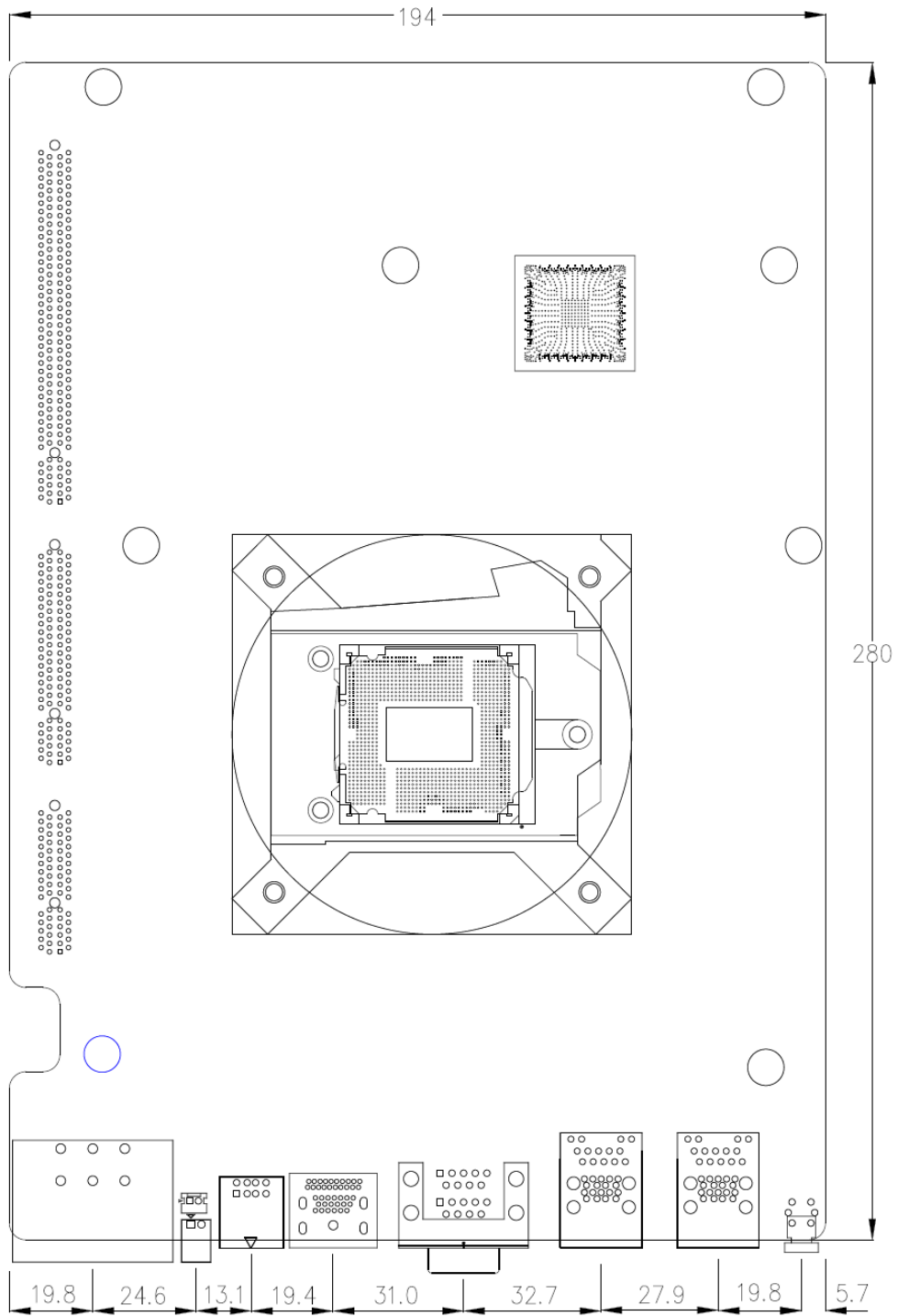
Figure 2.1: Motherboard Dimensions
