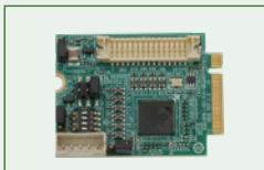
iDPM-LVDS-R10
