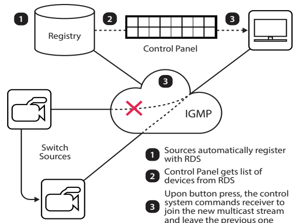
IS-04 and IS-05 System Diagram
